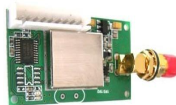
Gambar 5 RF Data Transceiver YS-1020ua
