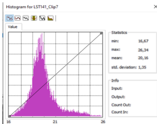
Gambar 3. Histogram LST 2014
