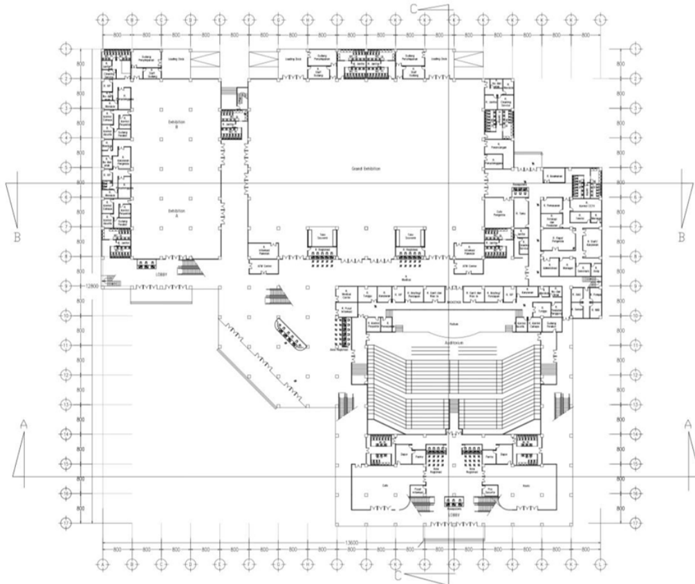
GAMBAR 10 Denah
