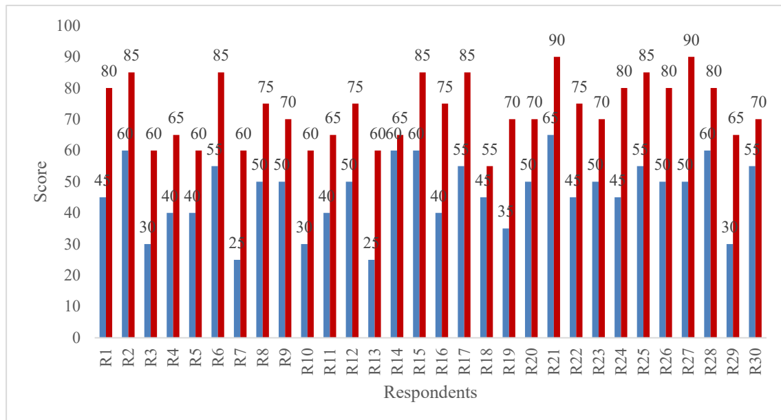
Figure 4. Pretest (blue) and posttest (red) scores for conceptual understanding indicators
