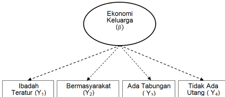
Gambar 4.5 Loading Factor Correlation (Dimension)
