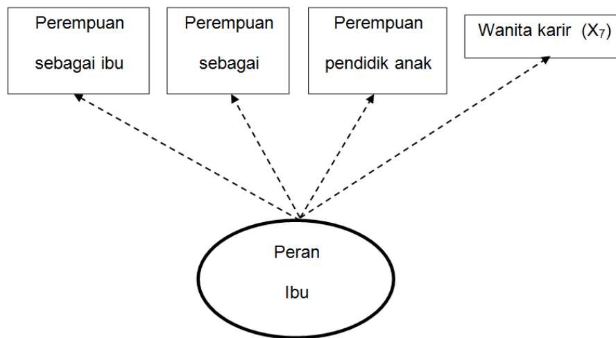
Gambar C.2 Loading Factor Correlation (Dimension)
